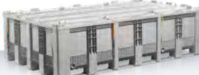
SB | 2988 L 50H/Y/.../NL/2139-250602/2630/1383 ① 2950 x 1850 x 790 mm ② 2965 x 1863 x 862 mm Max. gross weight: 1383 kg Standard colours: ■
