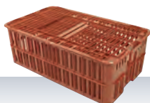
Poultry Transport Crate 90 L 840 × 495 × 295 mm On request Standard colours: ■
